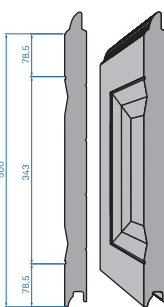
kazeta
